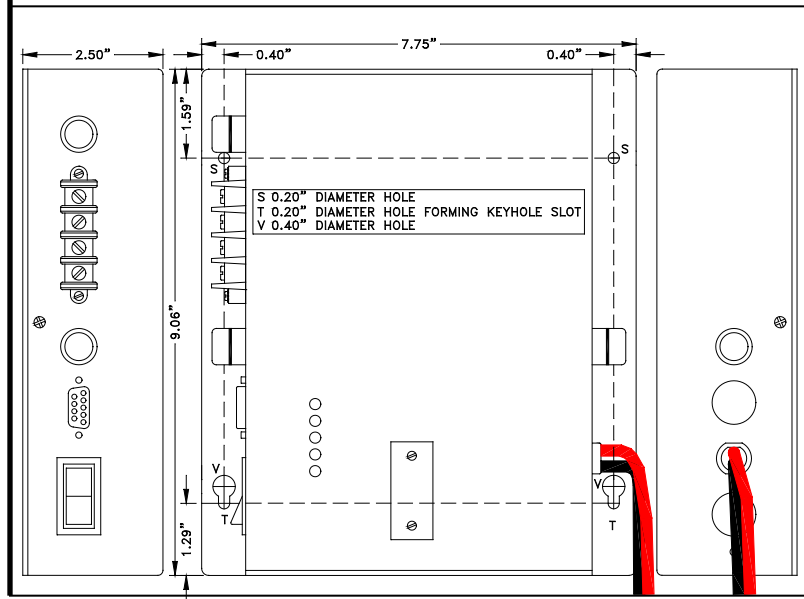
Mechanical Diagram
